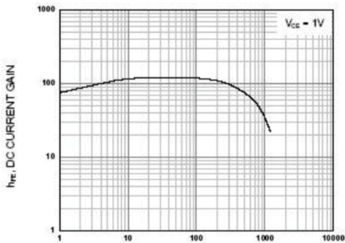
COLLECTOR CURRENT I_c (mA)
