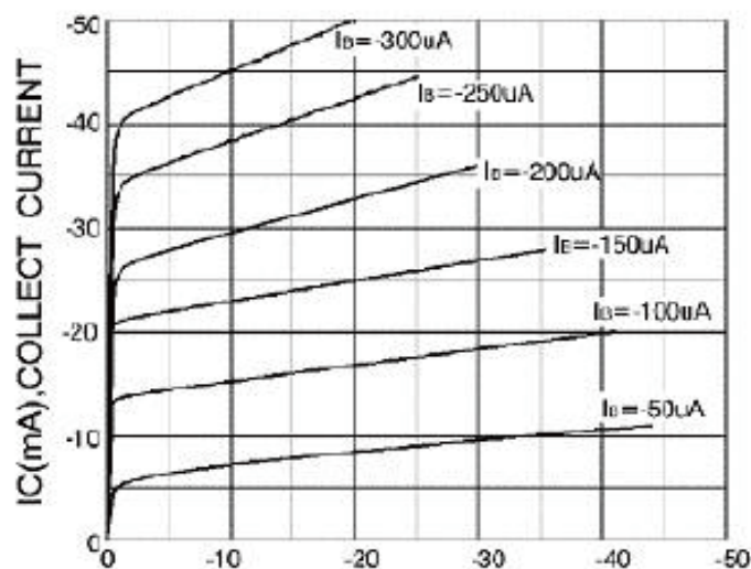
COLLECTOR-EMITTER VOLTAGE V_{CE} (V)
