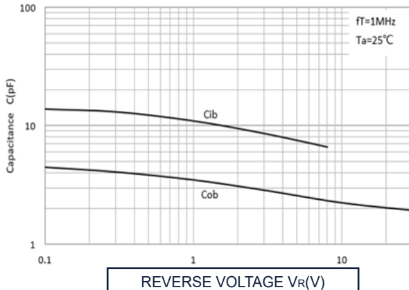
C_{ob}/C_{ib}-V_{CB}/V_{EB}
