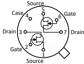
TO-78 Bottom View
