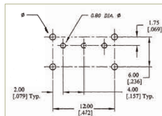
P.C. MOUNTING
