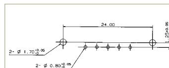
P.C. MOUNTING
