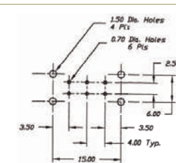
P.C. MOUNTING
