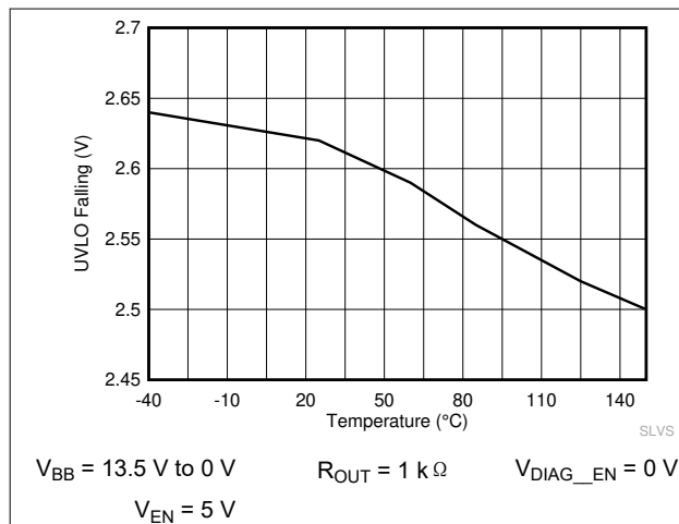
图 7-1. Falling Undervoltage Lockout ( V_{UVLOF} ) vs Temperature
