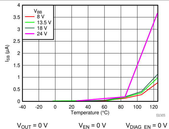
图 7-2. Standby Current ( I_{SB} ) vs Temperature
