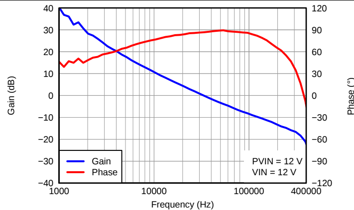
图 5. V_{OUT}=1.2\text{ V} , I_{OUT}=3\text{ A} , C_{OUT1}=47\text{ }\mu\text{F} ceramic, C_{OUT2}=330\text{ }\mu\text{F} POSCAP, f_{SW}=480\text{ kHz}
