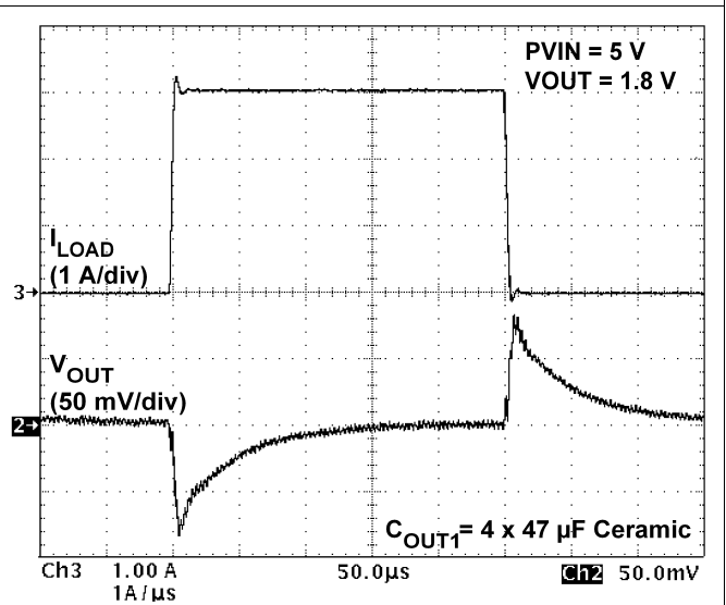
图 20. PVIN = 5V, VOUT = 1.8V, 3A Load Step
