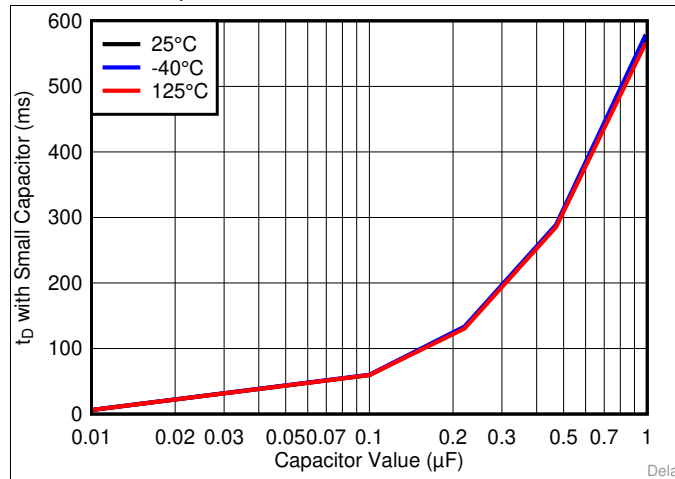
图 7. Reset Time Delay vs Small Capacitor Values
