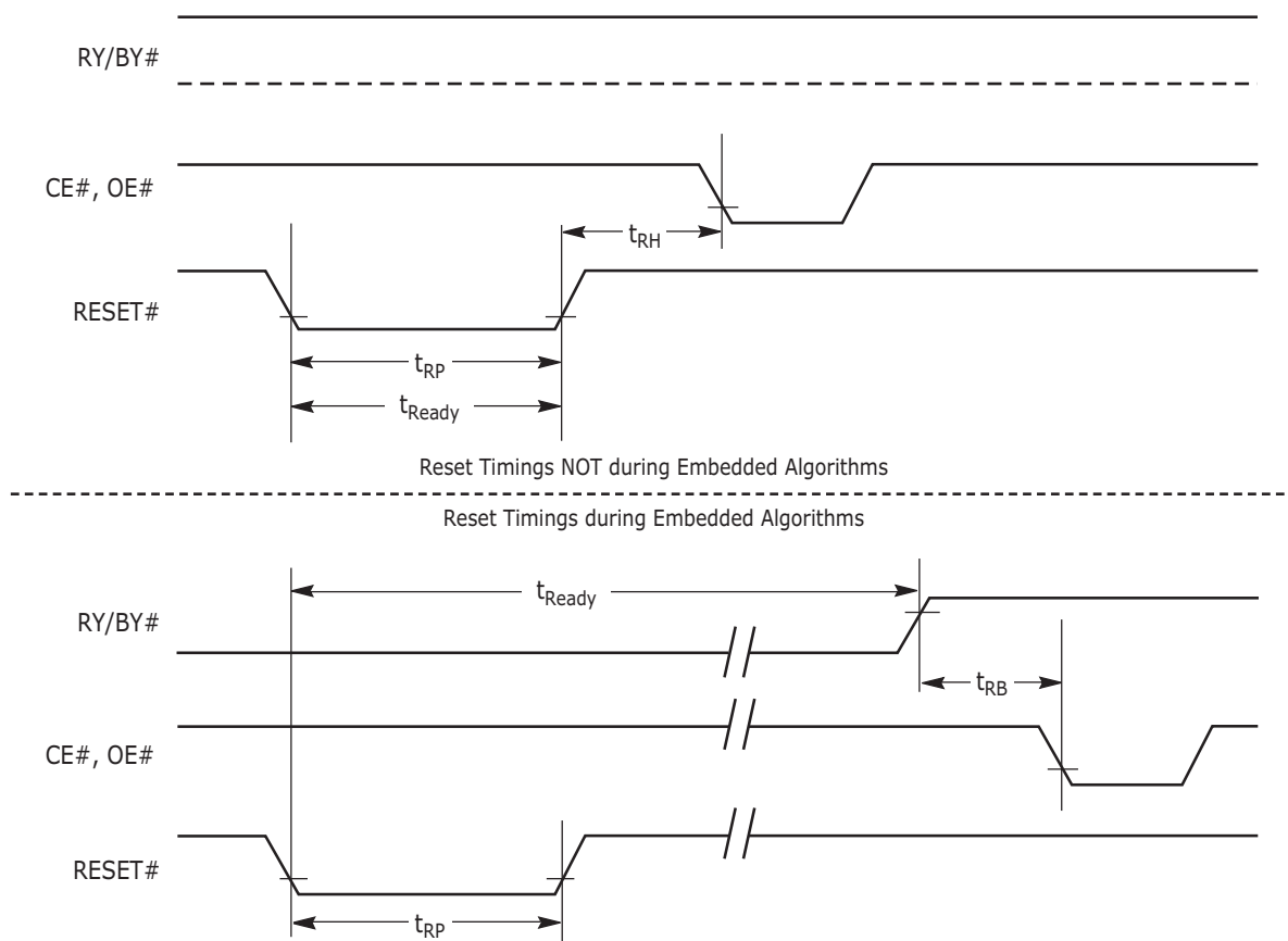
Figure I4. RESET# Timings
