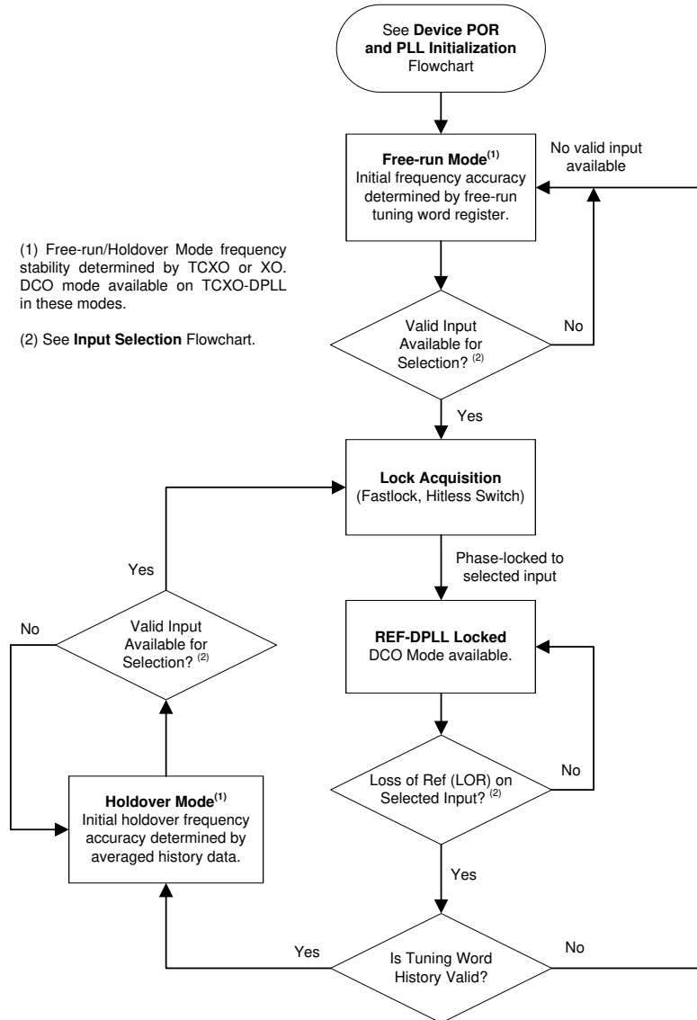
图 7-39. PLL Operating Mode
