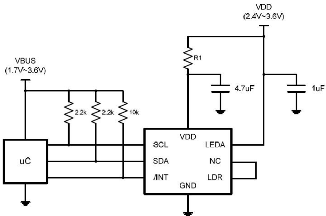
ZC-SAPMTK311 Typical Application Circuit with Only One Supply Voltage
