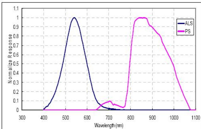
Spectral Response
