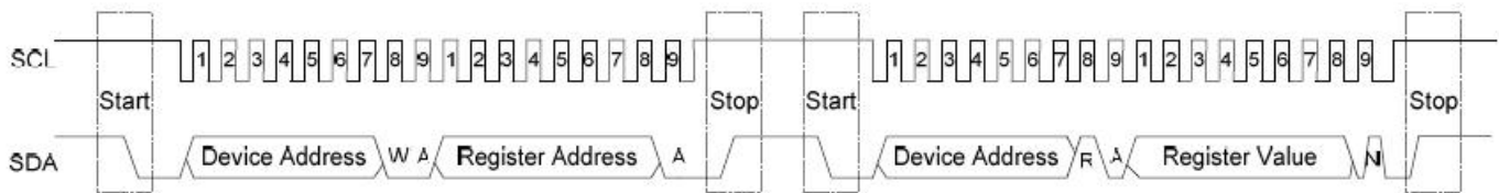
Read Data
