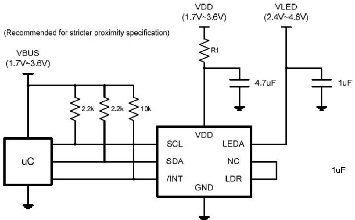
ZC-SAPMTK311 Typical Application Circuit with Independent VDD and VLED Supply Voltage
