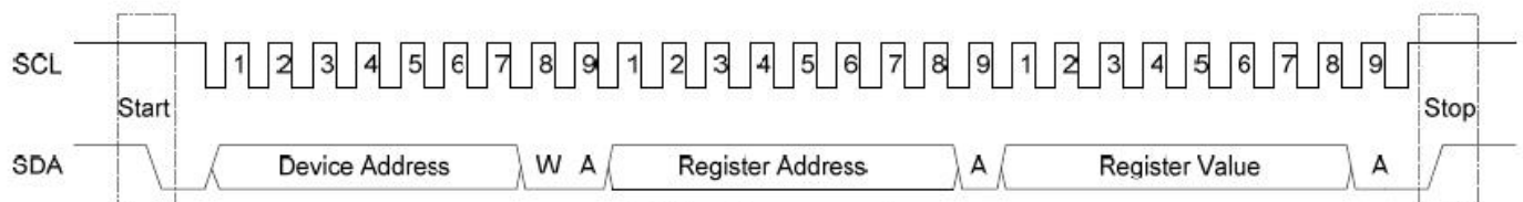
Write Command
