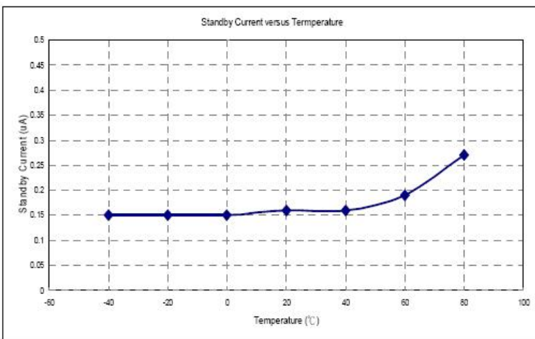
I_{SD} versus Temperature @ VDD = 2.8V, Halogen
