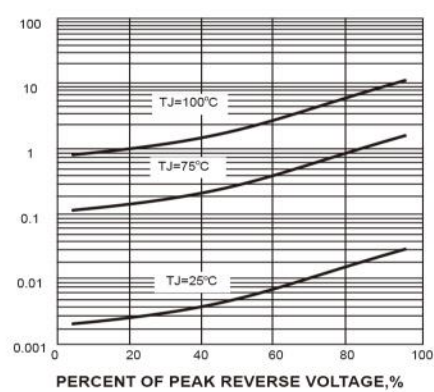
FIG. 4-TYPICAL REVERSE CHARACTERISTICS
