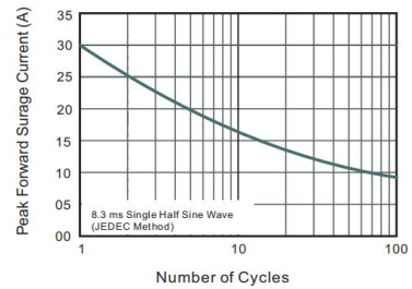
Fig.4 Maximum Non-Repetitive Peak Forward Surge Current
