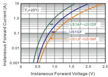
Fig.3 Typical Forward Characteristics
