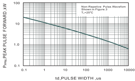
Fig.1 Peak Pulse Power Rating Curve
