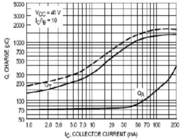
Figure 2 Charge Data
