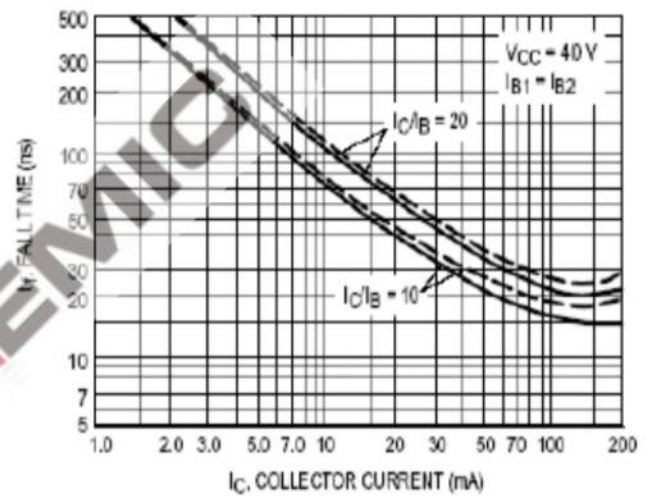
Figure 4 Fall Time
