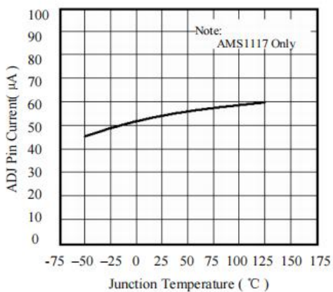
Figure 8. ADJ Pin Current VS. Temperature
