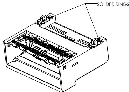
V95-ADZ01-000021T (BELLY TO BELLY APPLICATION)
