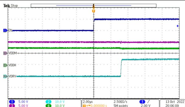
Figure 9-7. Three-Wire Mode, f_{EN} = 10\text{ kHz} , TPSI3052-Q1
