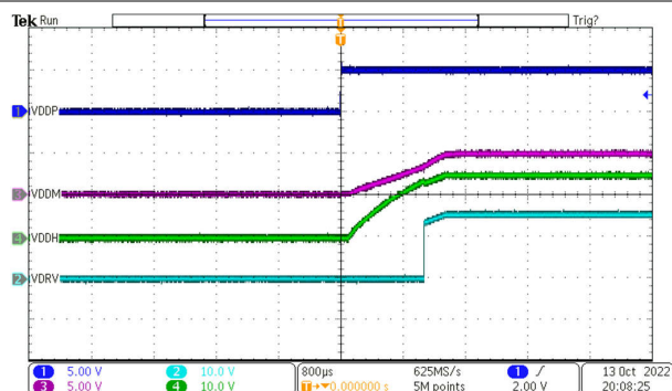
Figure 9-6. t_{LH\_VDRV} , Three-Wire Mode, TPSI3052-Q1
