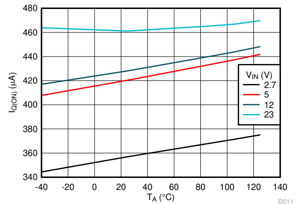
图 7-3. IN Quiescent Current vs Temperature
