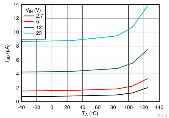
图 7-5. IN Shutdown Current vs Temperature
