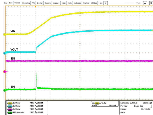
图 7-27. Start-Up with IN Supply
