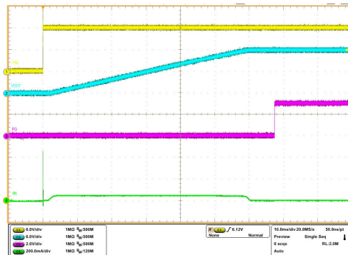
图 7-26. Start-Up with Enable
