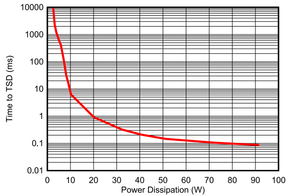
图 7-24. Time to Thermal Shut-Down During Inrush State
