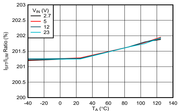
图 7-15. Scalable Fast-Trip Threshold: Current Limit Threshold ( I_{LIM} ) Ratio vs Temperature
