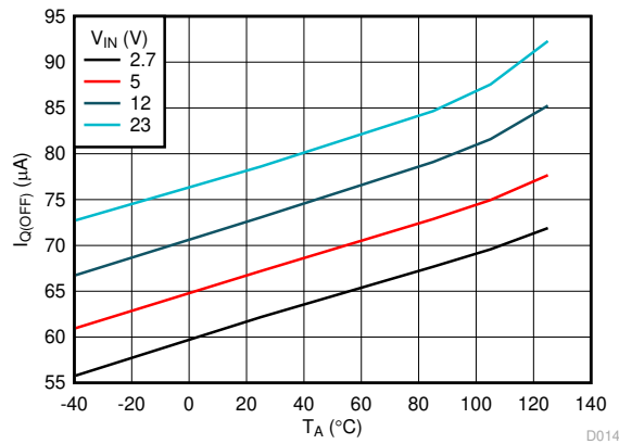
图 7-4. IN OFF State (UVLO) Current vs Temperature
