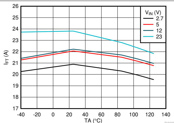
图 7-16. Steady State Fixed Fast-Trip Current Threshold vs Temperature
