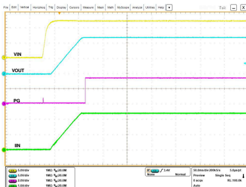
图 7-28. IN Hot-Plug
