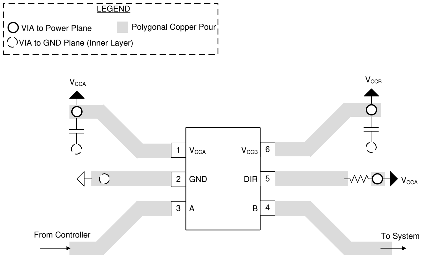
图 8-5. PCB Layout Example
