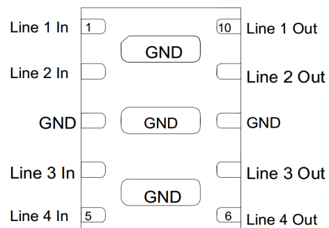
Pin Schematic
