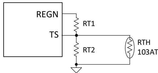
图 9-5. TS Resistor Network
