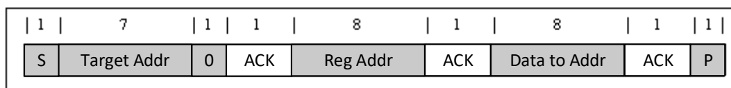
图 9-16. Single Write
