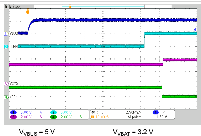
图 10-2. Power-Up with Charge Disabled
