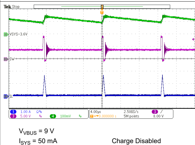
图 10-5. PFM Switching in Buck Mode
