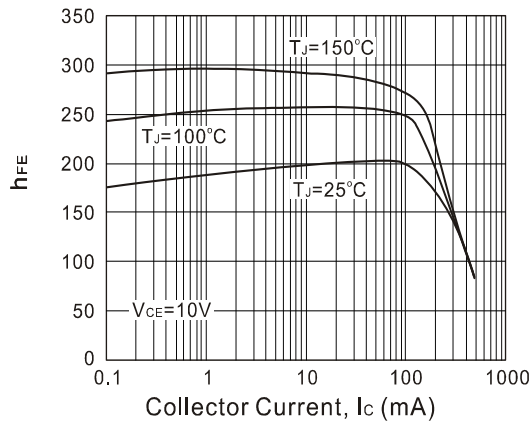
Fig. 3. Typical h_{FE} vs Collector Current
