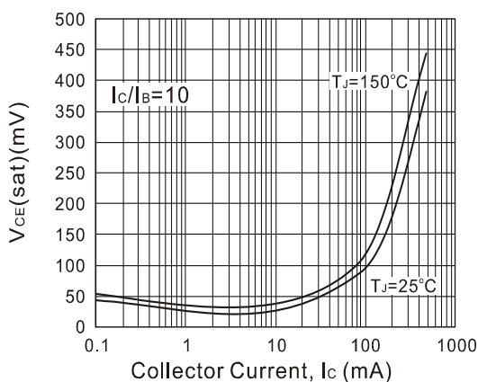
Fig. 5. Typical V_{CE(sat)} vs Collector Current
