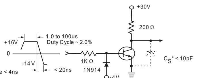
Fig. 2 Turn-Off Time
