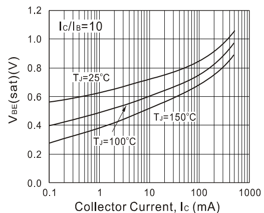
Fig. 6. Typical V_{BE(sat)} vs Collector Current
