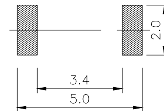
PCB. WELDING DRAWING
