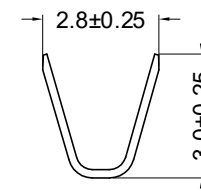
SECTION F-F
