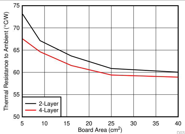
图 6-9. Package Thermal Resistance vs Board Copper Area, No Air Flow
