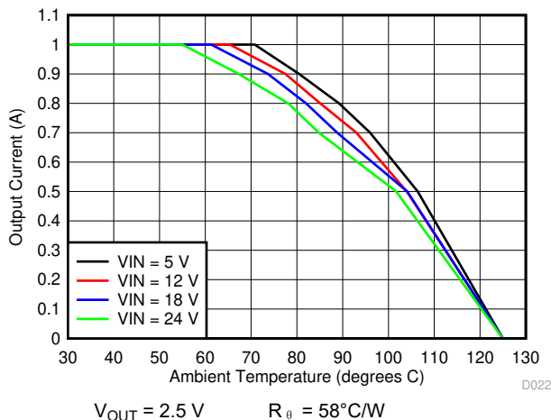
图 6-19. Ambient Temperature vs Output Current
