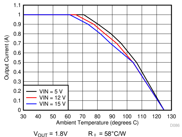
图 6-18. Ambient Temperature vs Output Current
