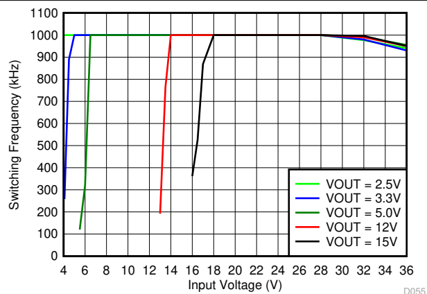
图 6-31. Switching Frequency vs Input Voltage for Adjustable Output Options at Full Load
