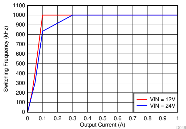
图 6-25. Auto PFM Mode Switching Frequency vs Output Current
