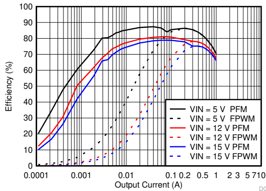
图 8-36. Efficiency for V_{OUT} = 1.8\text{ V}
