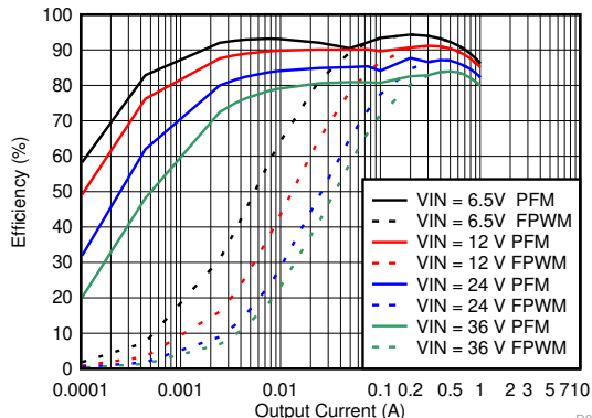
图 8-42. Efficiency for V_{OUT} = 5\text{ V}
