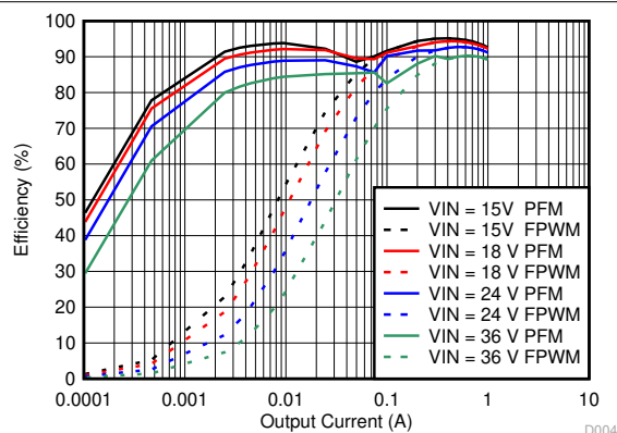
图 8-18. Efficiency
