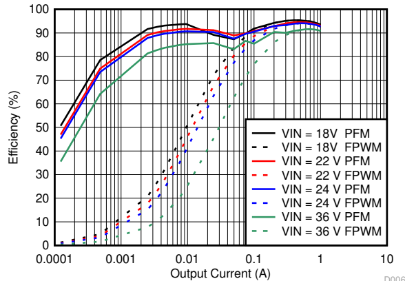
图 8-24. Efficiency
