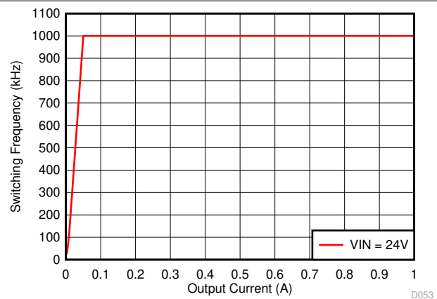
图 6-28. Auto PFM Mode Switching Frequency vs Output Current
