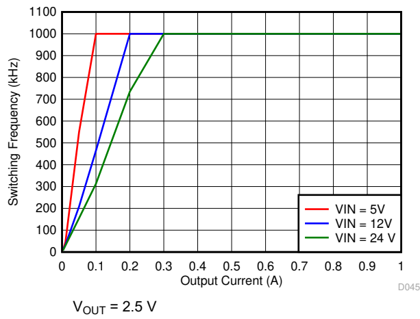
图 6-24. Auto PFM Mode Switching Frequency vs Output Current
