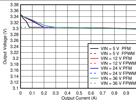
图 8-45. Line and Load Regulation for V_{OUT} = 3.3\text{ V}
