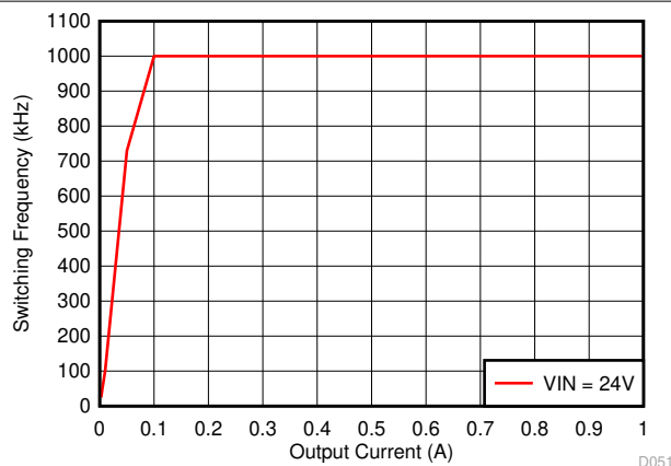
图 6-29. Auto PFM Mode Switching Frequency vs Output Current
