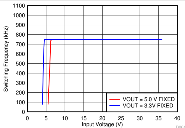
图 6-32. Switching Frequency vs Input Voltage for Fixed Output Options at Full Load
