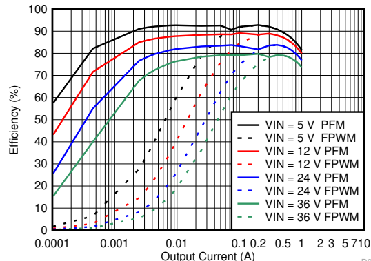
图 8-43. Efficiency for V_{OUT} = 3.3\text{ V}
