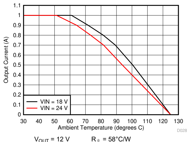
图 6-22. Ambient Temperature vs Output Current
