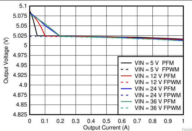
图 8-10. Line and Load Regulation
