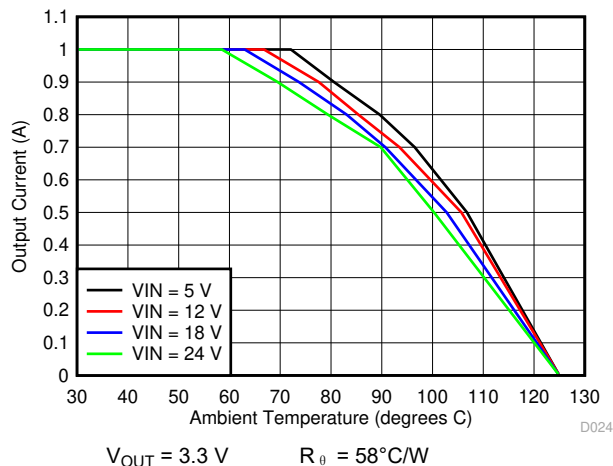
图 6-20. Ambient Temperature vs Output Current
