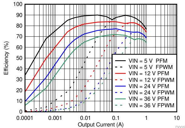
图 8-30. Efficiency
