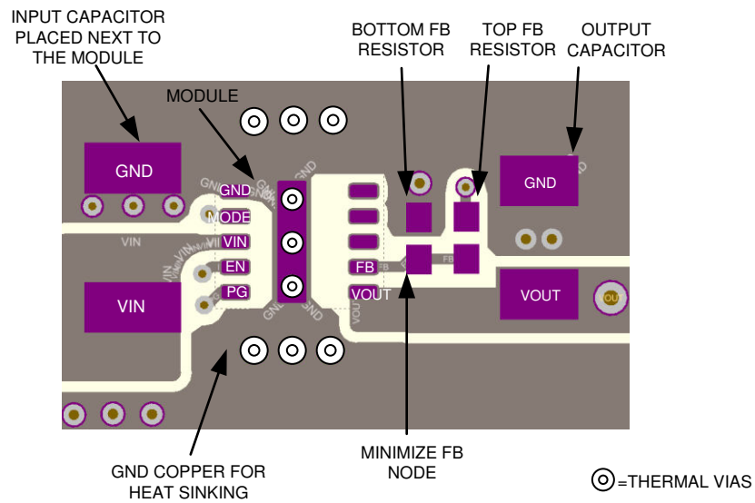
图 8-50. Layout Example With Adjustable Output Version
