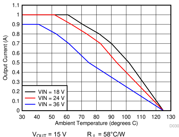
图 6-23. Ambient Temperature vs Output Current
