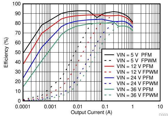
图 8-12. Efficiency
