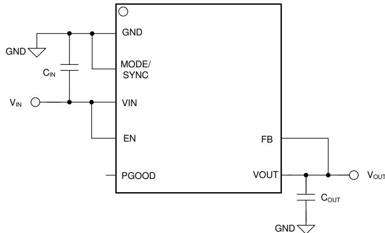
图 8-1. Fixed 5-V or 3.3-V Typical Application Circuit
