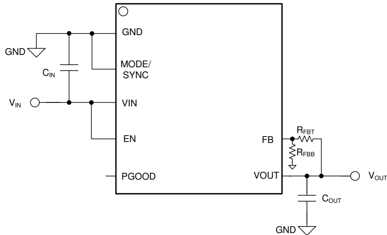
图 8-4. Adjustable 1.2-V to 15-V Output Typical Application Circuit
