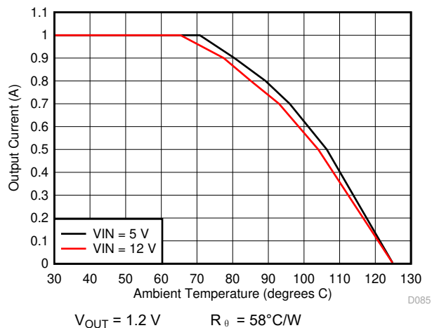
图 6-17. Ambient Temperature vs Output Current
