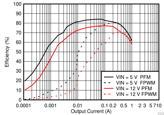
图 8-37. Efficiency for V_{OUT} = 1.2\text{ V}
