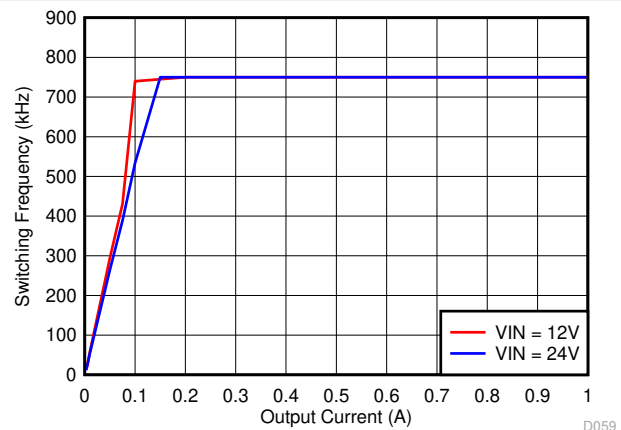
图 6-26. Auto PFM Mode Switching Frequency vs Output Current
