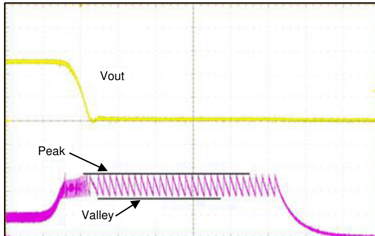
图 7-1. Current Limit Operation During Output Short Circuit
