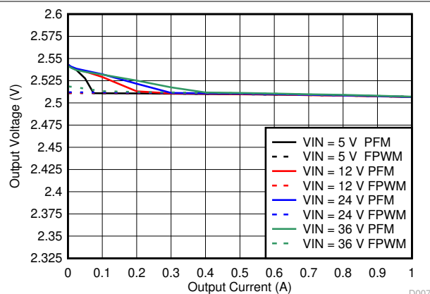
图 8-34. Line and Load Regulation
