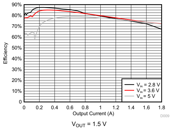
图 9-6. DCDC3 Efficiency
