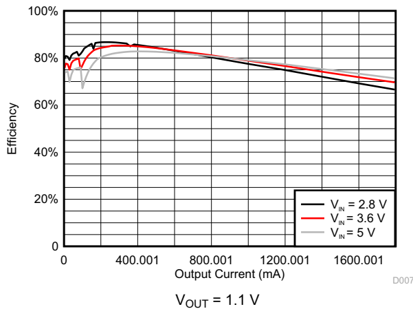
图 9-4. DCDC1/DCDC2 Efficiency
