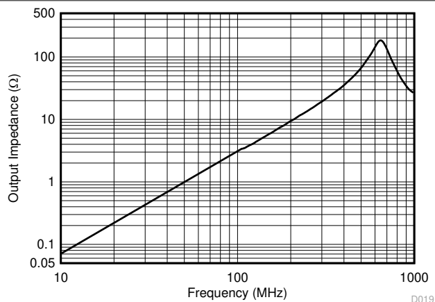
图 8-27. Output Impedance vs Frequency
