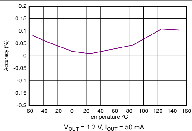
图 6-8. Accuracy vs Temperature
