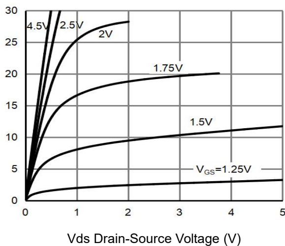
Figure 5 Output Characteristics
