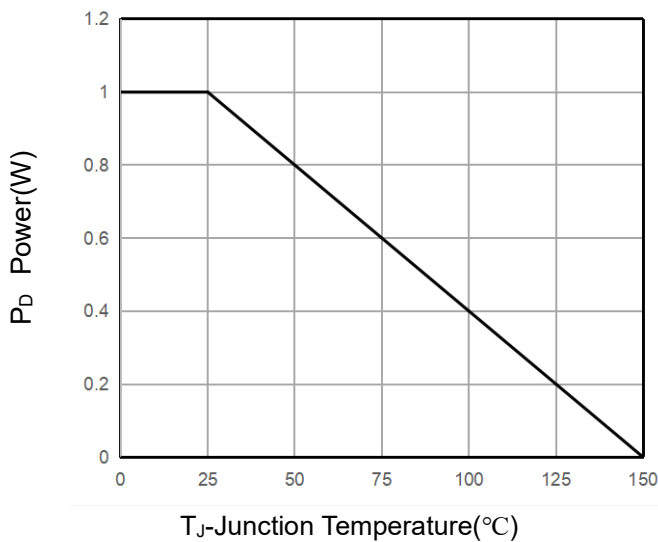
Figure 3 Power Dissipation
