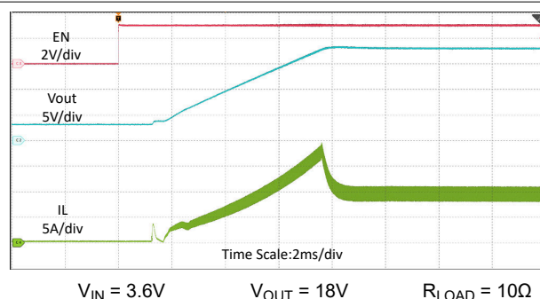
Figure 7-8. Start-up Waveforms
