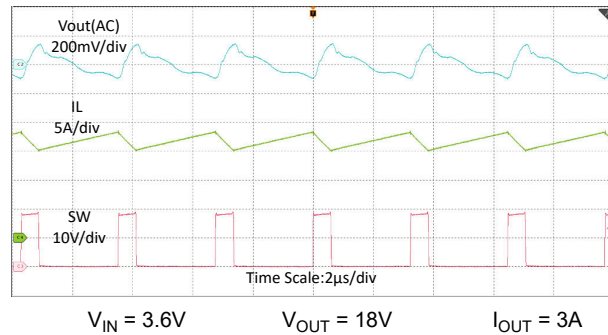
Figure 7-2. Switching Waveforms in 3A load PFM Mode
