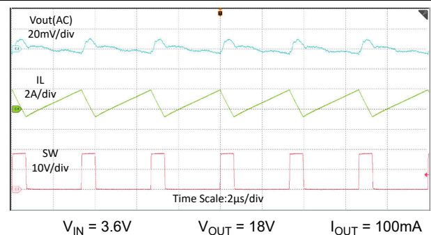
Figure 7-5. Switching Waveforms in 100mA load FPWM Mode
