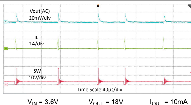
Figure 7-6. Switching Waveforms in 10mA load PFM Mode
