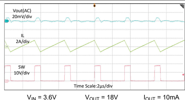
Figure 7-7. Switching Waveforms in 10mA load FPWM Mode
