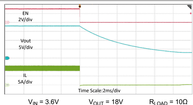
Figure 7-9. Shutdown Waveforms
