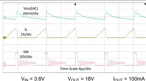
Figure 7-4. Switching Waveforms in 100mA load PFM Mode
