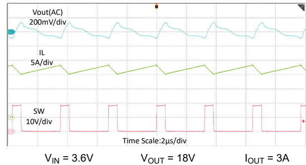
Figure 7-3. Switching Waveforms in 3A load FPWM Mode
