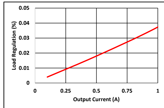
Fig. 4 Load Regulation
