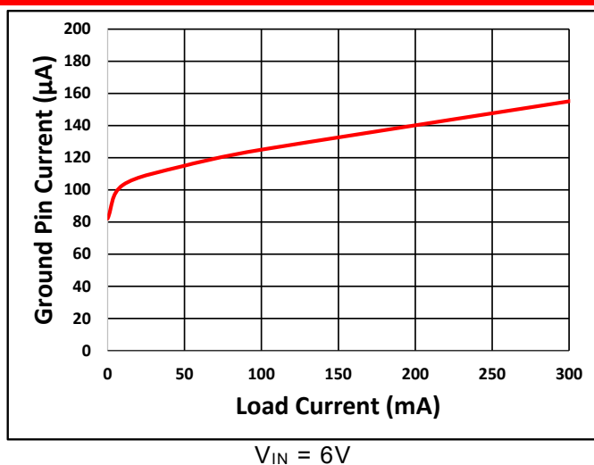
Fig. 5 Ground Current vs Load Current
