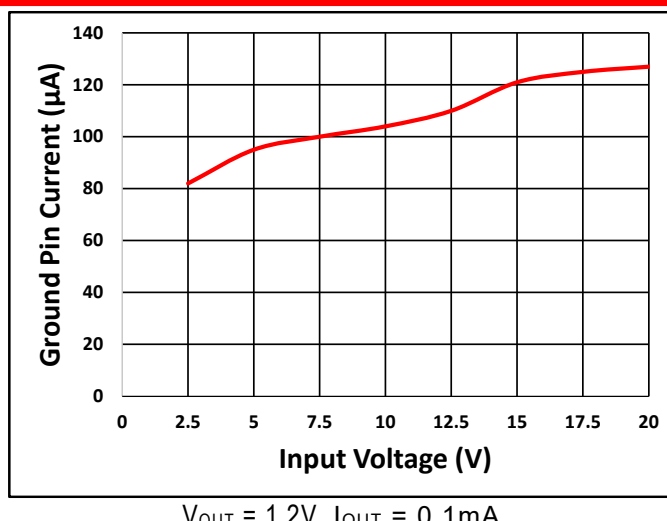
Fig. 6 Ground Current vs Input Voltage
