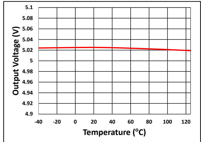
Fig. 4 Output Voltage vs Temperature
