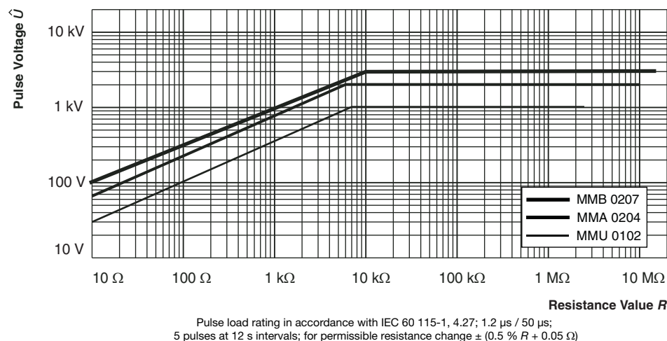
1.2 / 50 Pulse
