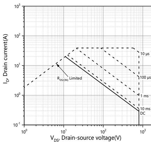
Figure 11. Safe operation area T_C=25\text{ }^{\circ}\text{C}
