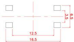
PCB. 焊接图 PCB.WELDING DRAWING
