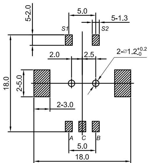
P.C.B. mounting hole detail
