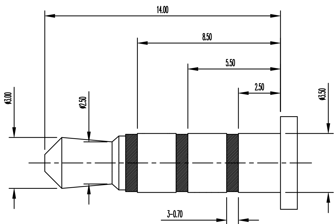
(φ3.50mm 4 POLE PLUG DETAIL DRAWING)
