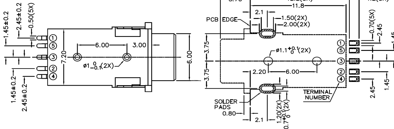
RECOMMEND PCB LAYOUT (TOP VIEW)
