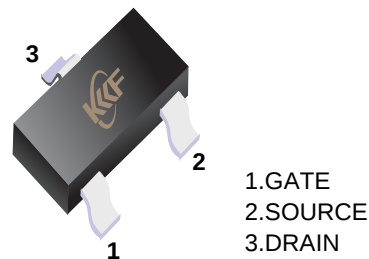
■ Simplified outline(SOT-523)
