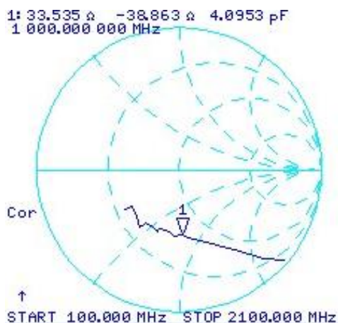
S_{22e} -FREQUENCY
