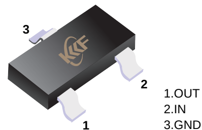
■ Simplified outline(SOT-23)
