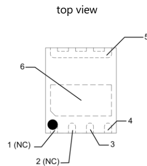
Package Outline
