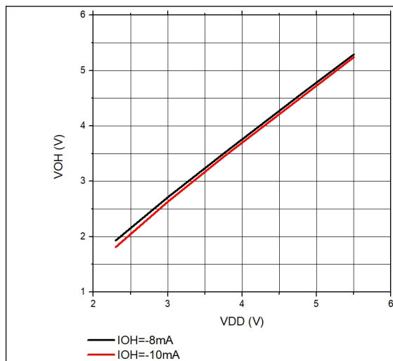
Figure 5.1. V_{OH} versus Supply Voltage
