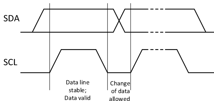
Figure 8.1. Bit transfer
