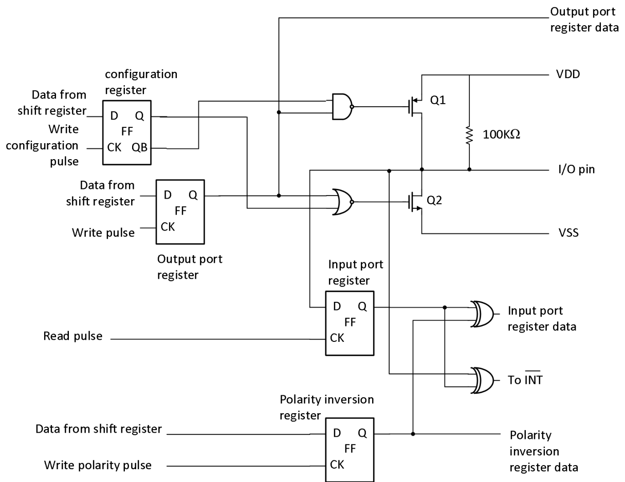
Figure 6.2. Simplified schematic of I/Os
