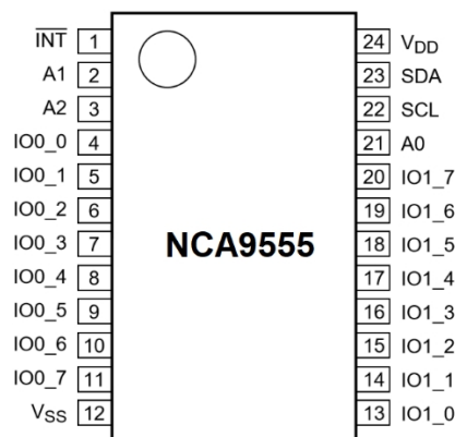
Figure 1. NCA9555 Block Diagram
