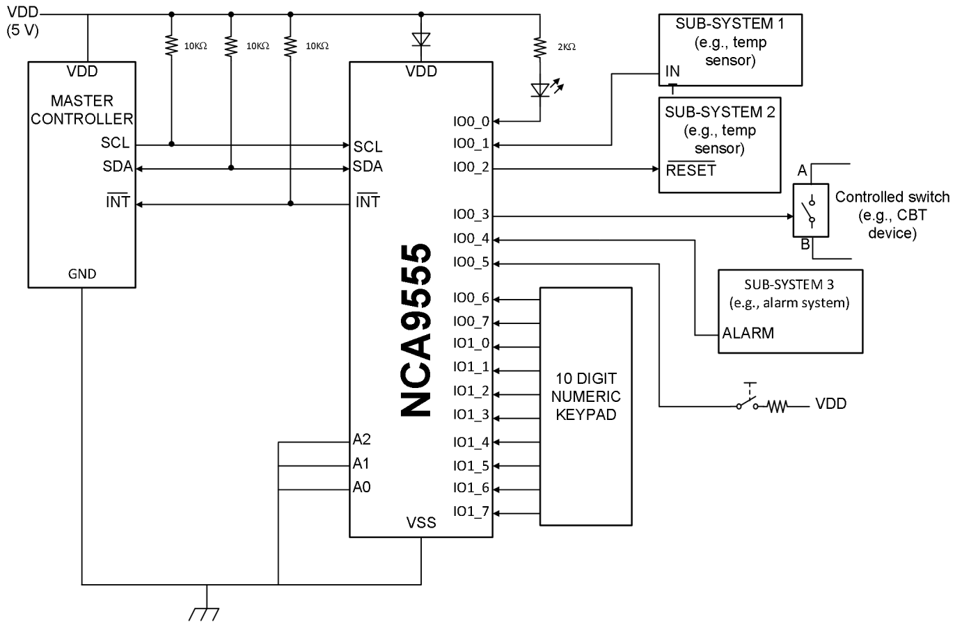
Figure 9.1. Typical application
