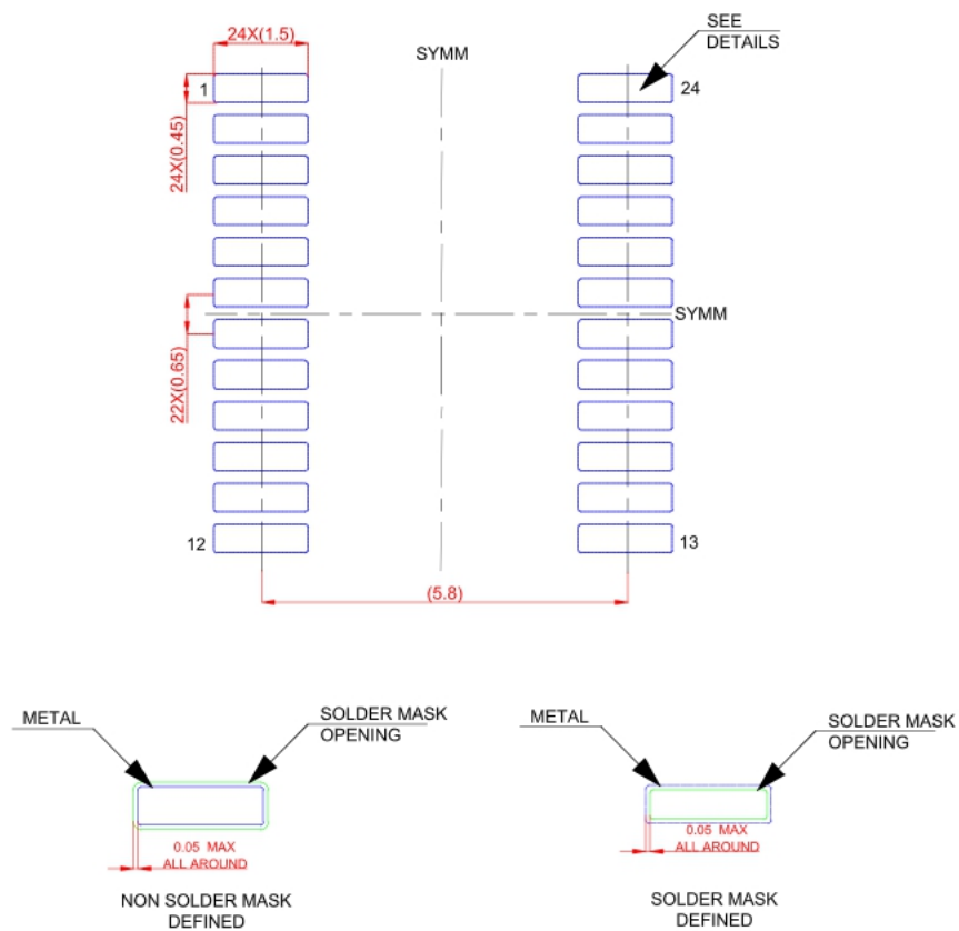
Figure 11.2.TSSOP24 Package Board Layout Example (unit:mm)
