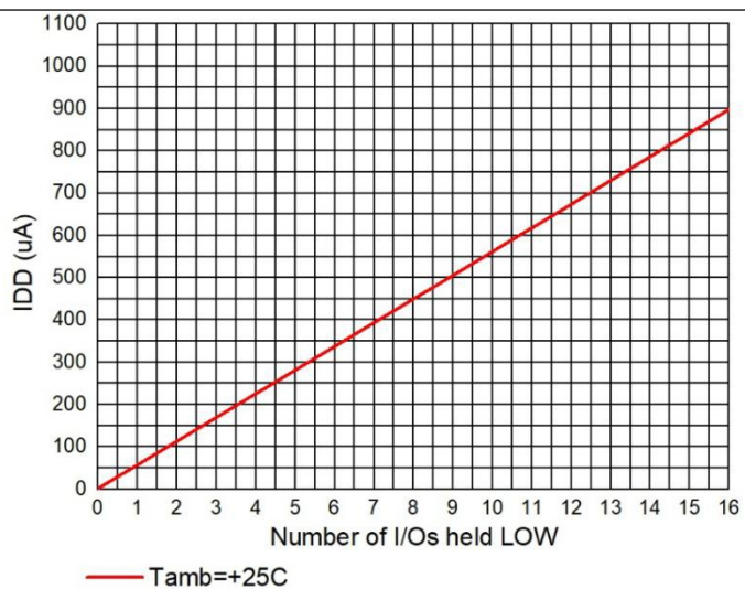
Figure 5.2. I_{DD} versus number of I/Os held LOW
