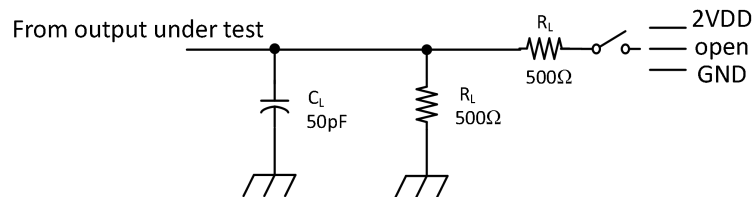
Figure 10.2. Load circuit
