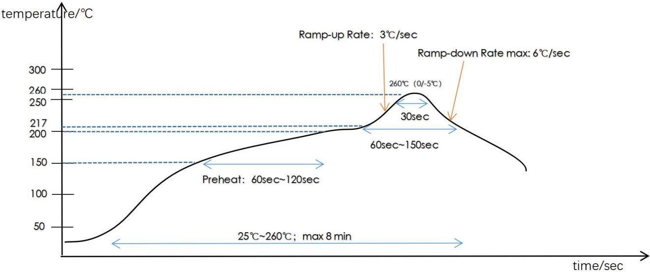
Figure24: Recommended Temperature(PB-Free)
