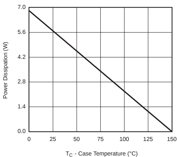
Power, Junction-to-Foot
