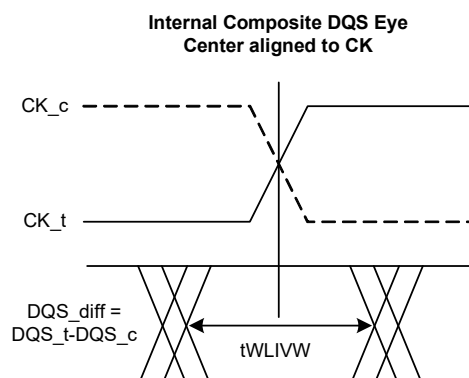
Figure 110 - DQS_t/DQS_c and CK_t/CK_c at DRAM Latch
