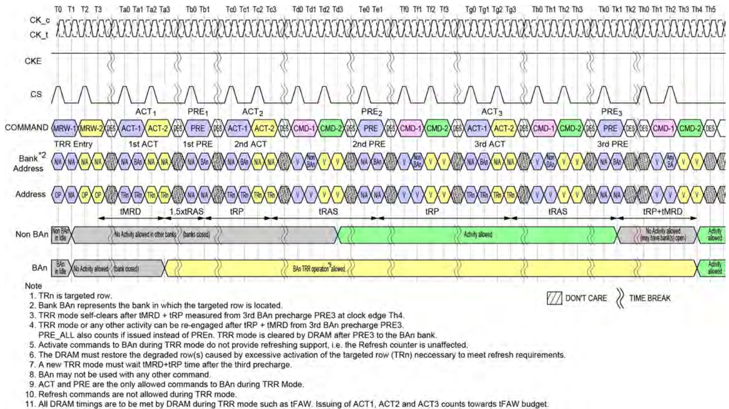
Figure 161 - TRR Mode Timing Example
