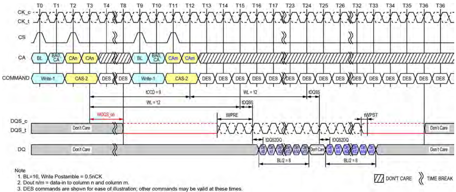
Figure 46 - Consecutive Writes Operation: t_{CCD} = \text{Min} + 1, 0.5nCK Postamble
