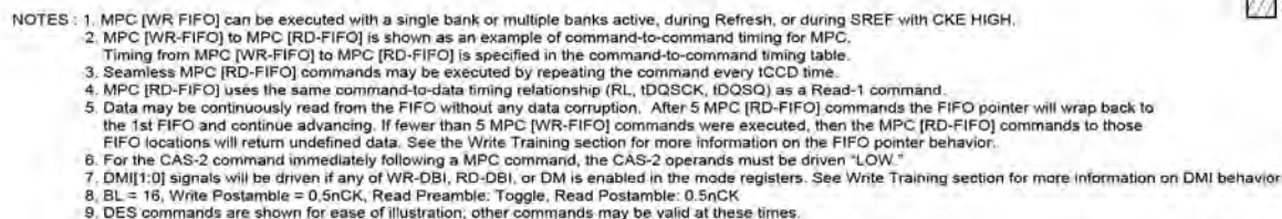
Figure 115 - MPC [Write FIFO] to MPC [Read FIFO] Timing
