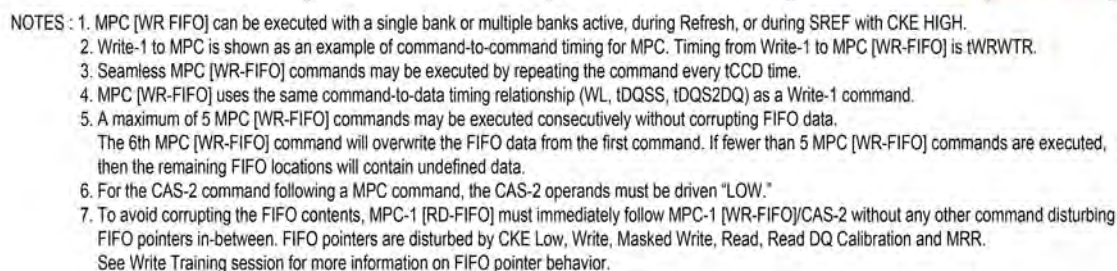
Figure 128 - MPC [WR FIFO] Operation : WPRE = 2nCK , tWPST = 0.5nCK
