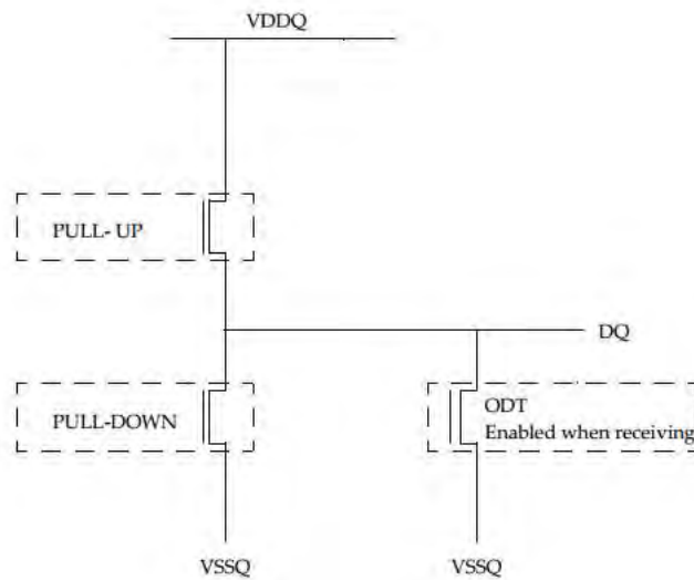
Figure 180 - LVSTL I/O Cell
