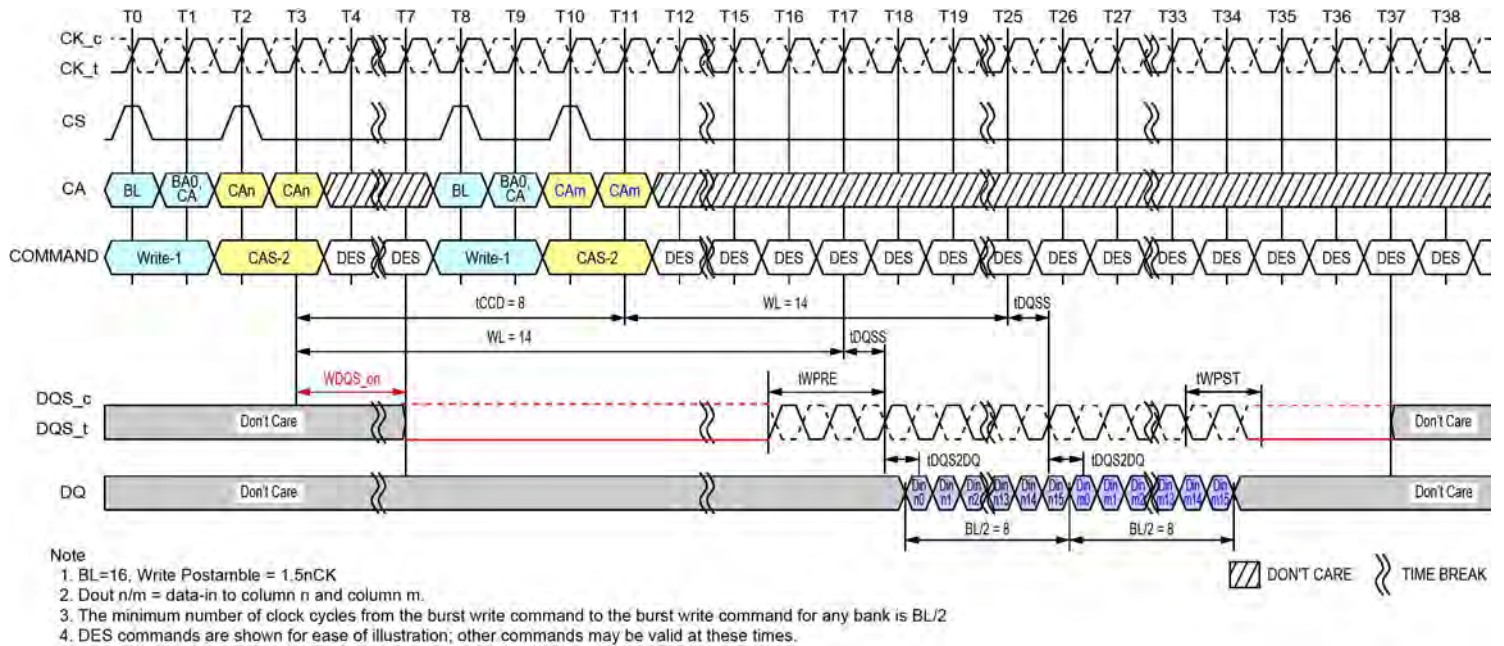
Figure 45 - Seamless Writes Operation: t_{CCD} = \text{Min}, 1.5nCK Postamble
