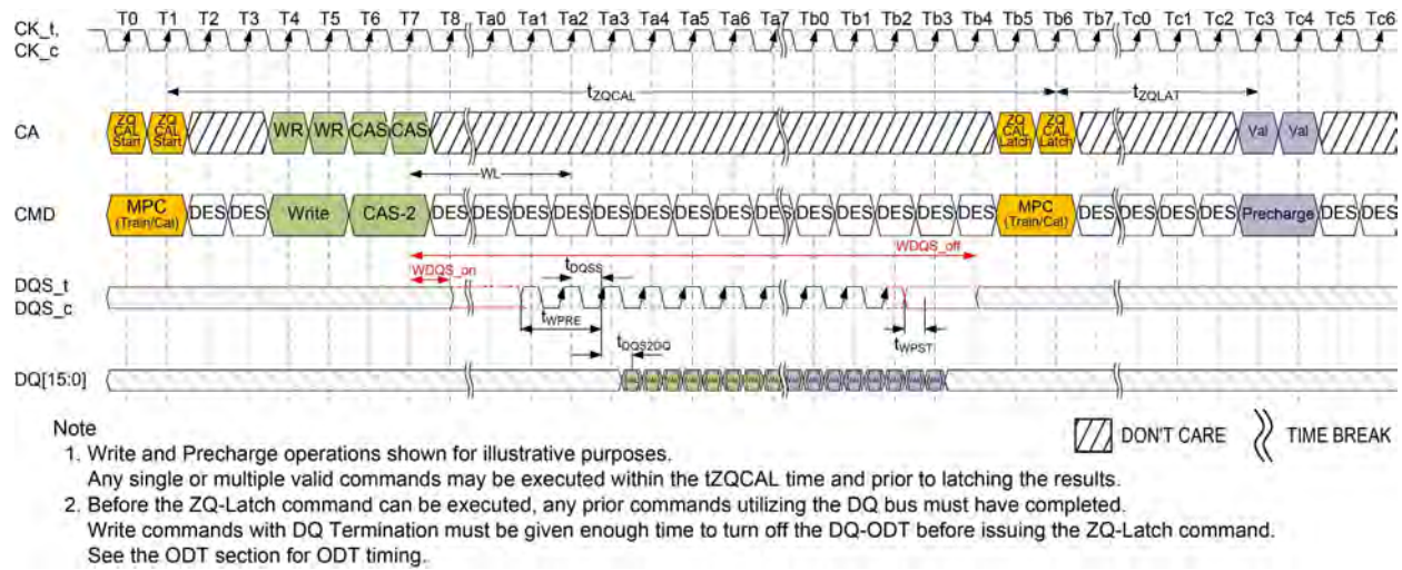
Figure 132 - ZQCal Timing
