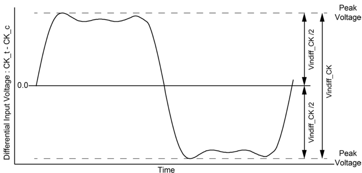
Figure 166 - CK Differential Input Voltage
