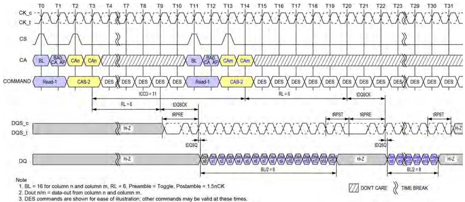
Figure 39 - Consecutive Reads Operation: t_{CCD} = \text{Min} + 3 , Preamble = Toggle, 1.5nCK Postamble
