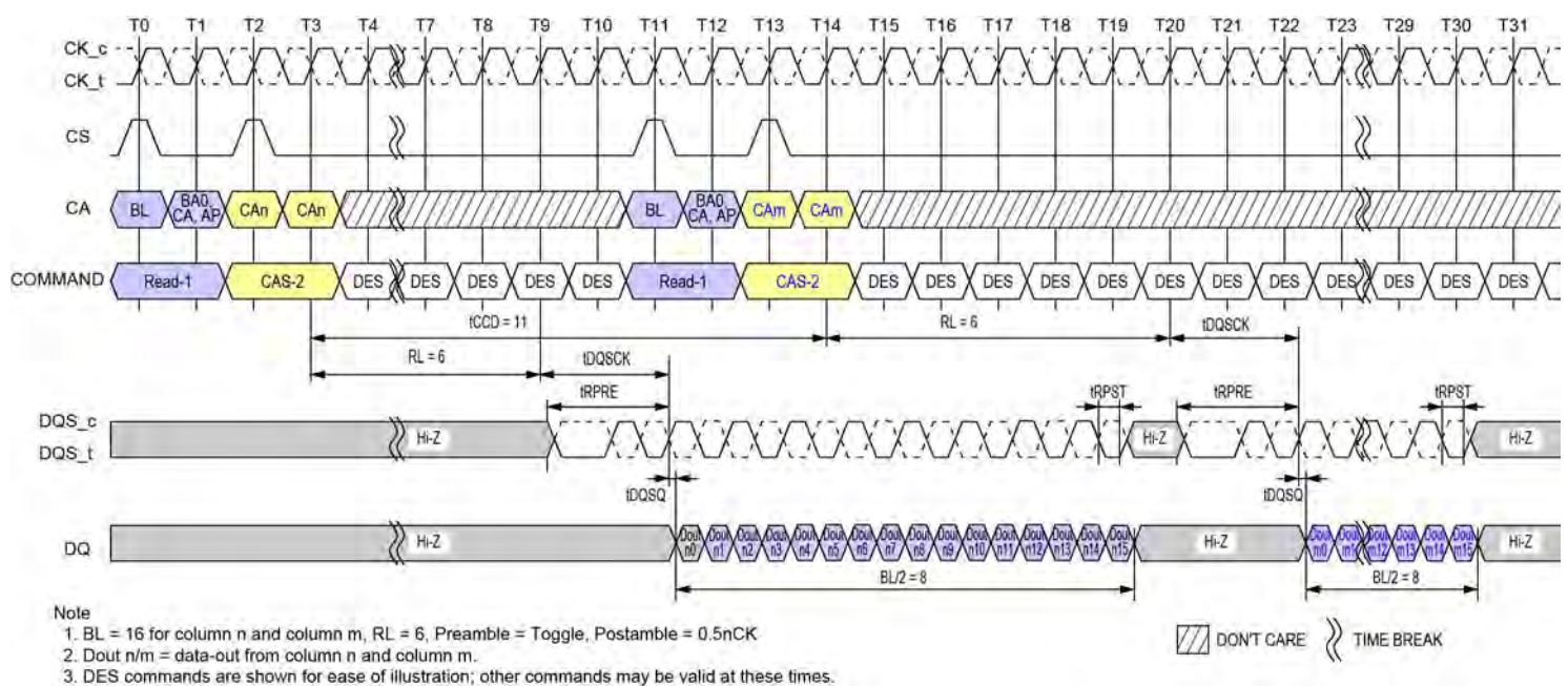
Figure 40 - Consecutive Reads Operation: t_{CCD} = \text{Min} + 3 , Preamble = Toggle, 0.5nCK Postamble
