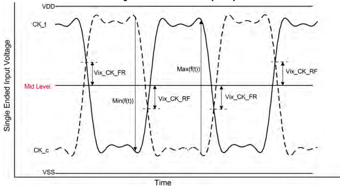
Figure 170 - Vix Definition (Clock)
