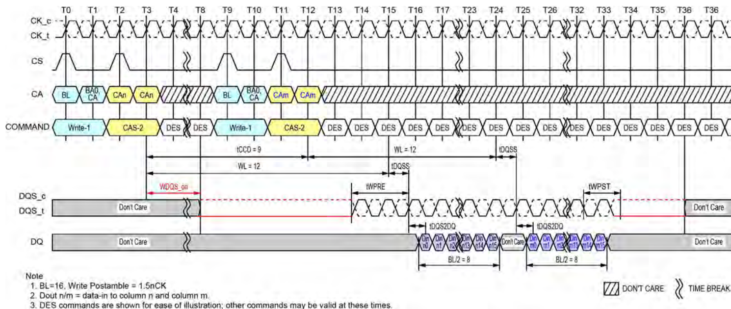
Figure 47 - Consecutive Writes Operation: t_{CCD} = \text{Min} + 1, 1.5nCK Postamble
