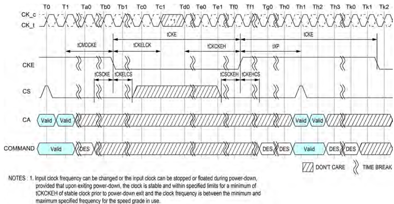
Figure 150 - Basic Power-down Entry and Exit Timing
