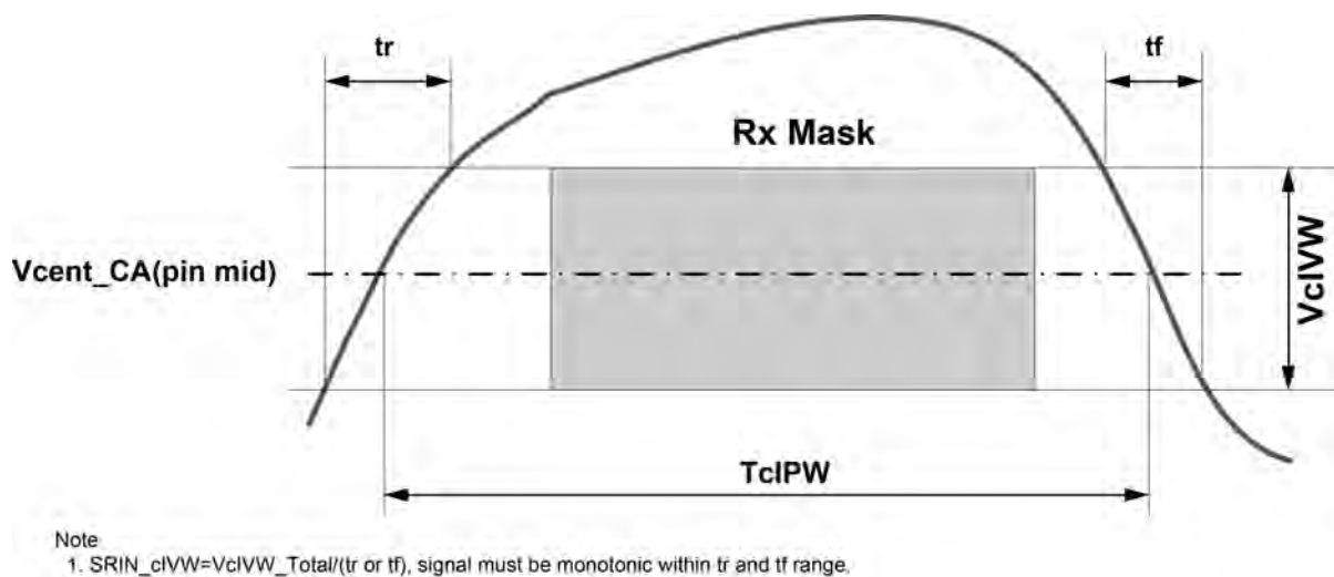
Figure 186 - CA TcIPW and SRIN_cIVW definition (for each input pulse)
