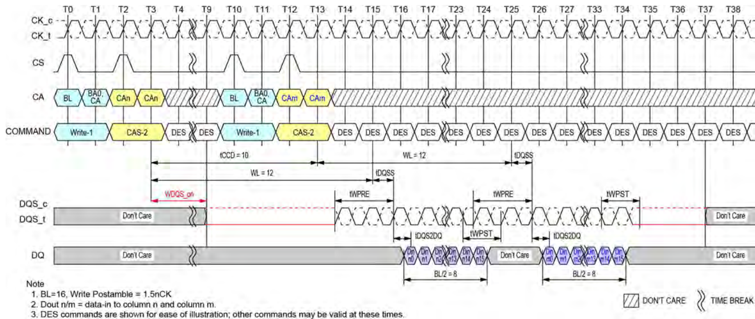
Figure 49 - Consecutive Writes Operation: t_{CCD} = \text{Min} + 2, 1.5nCK Postamble
