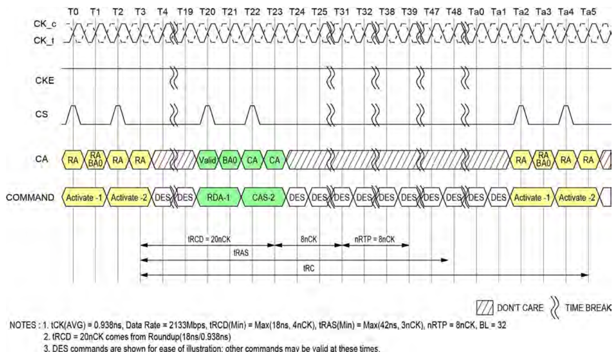
Figure 60 - Command Input Timing with RAS lock
