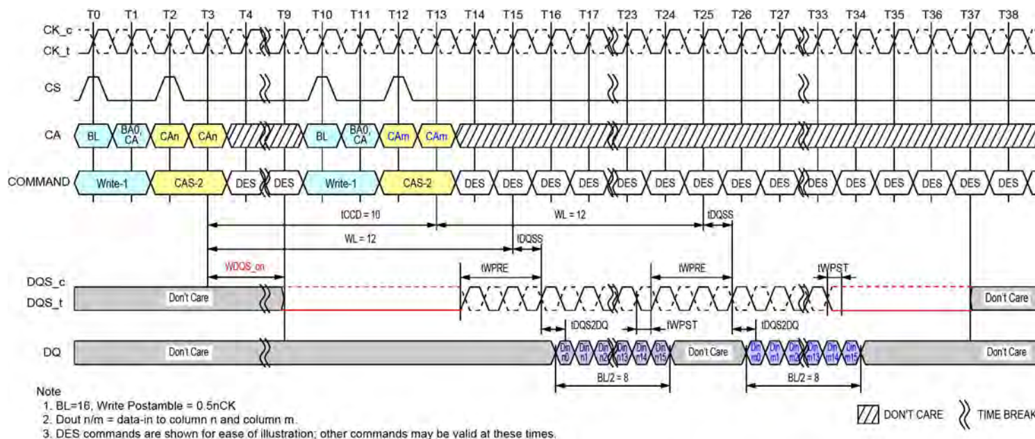
Figure 48 - Consecutive Writes Operation: t_{CCD} = \text{Min} + 2, 0.5nCK Postamble
