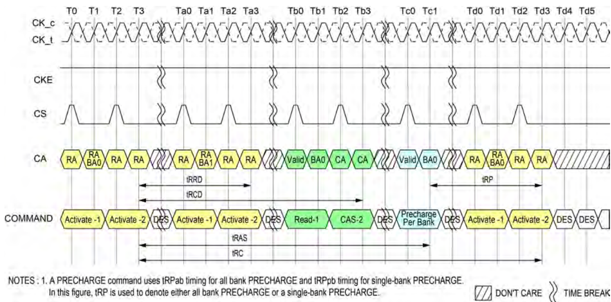
Figure 5 - Activate Command
