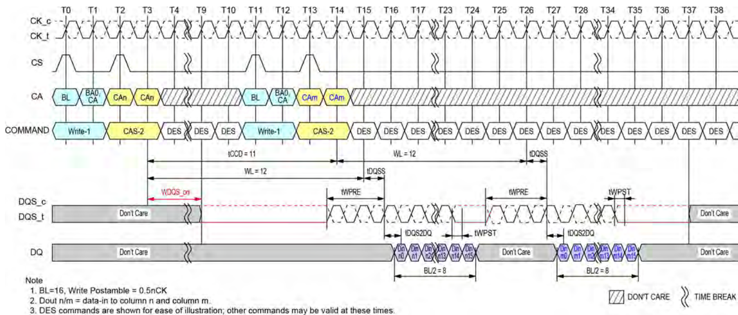
Figure 50 - Consecutive Writes Operation: t_{CCD} = \text{Min} + 3, 0.5nCK Postamble
