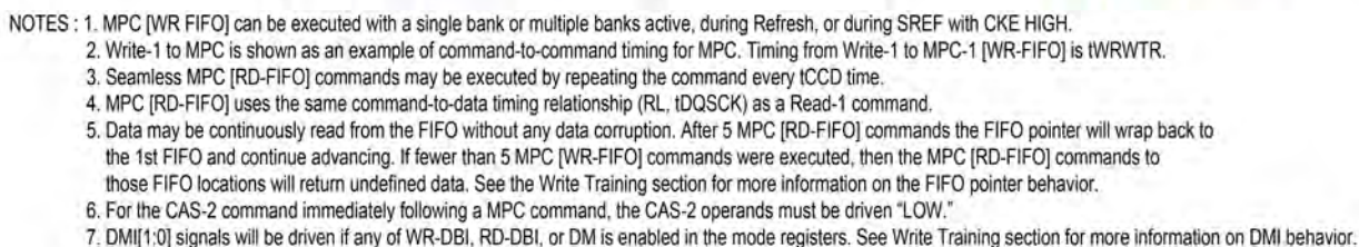
Figure 129 - MPC [RD FIFO] Read Operation (Shown with tWPRES=2nCK, tWPST=0.5nCK, tRPRES=toggling, tRPST=1.5nCK)
