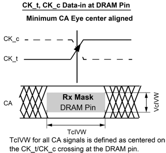
Figure 185 - CA Timing at the DRAM pins
