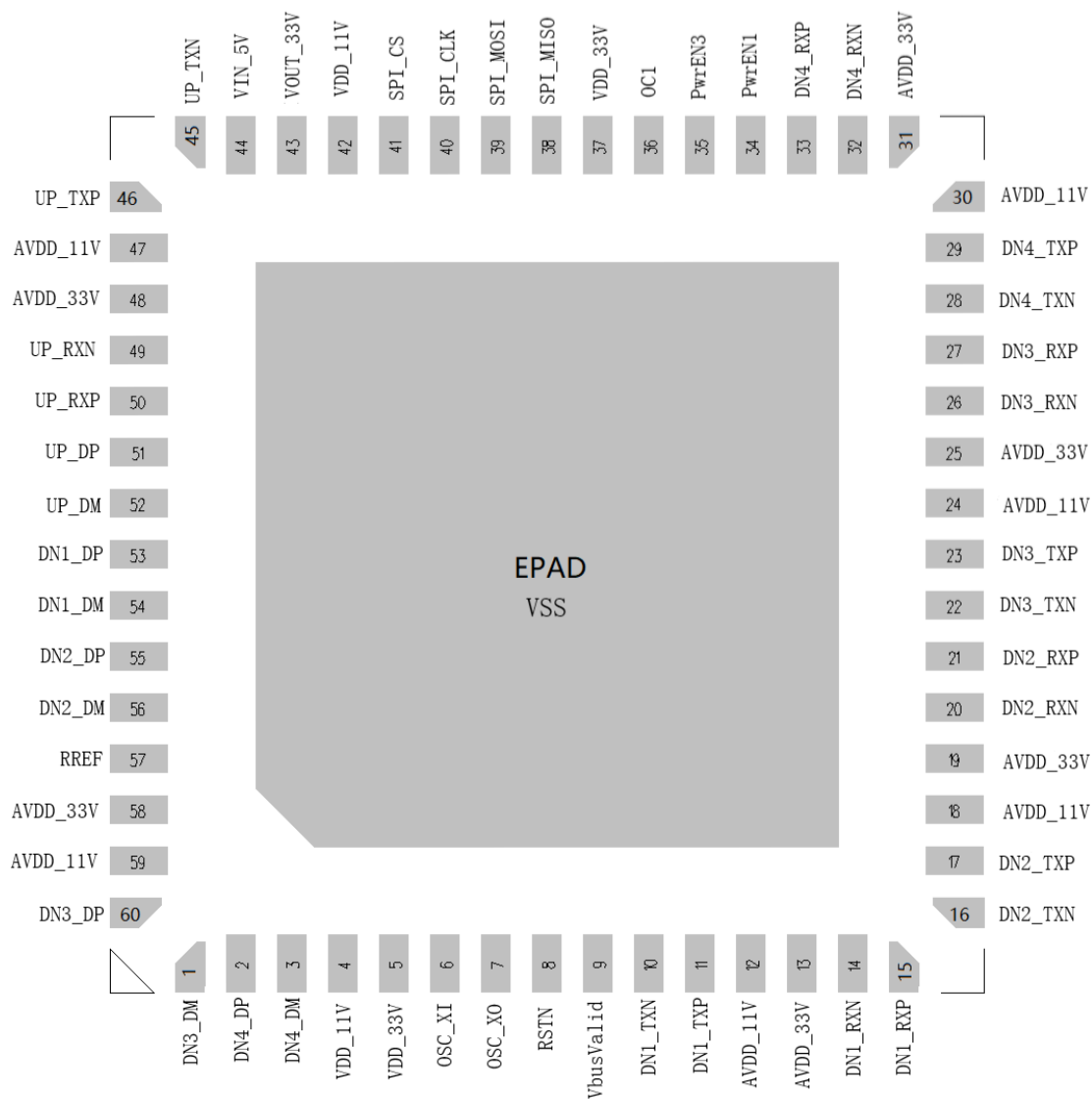
Figure 4.1 – SL6341 QFN60(6x6-0.35) Pin out Diagram
