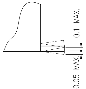
TERMINAL DETAIL (20/1)
